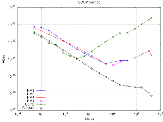
Fig. 3. Allan deviation plot of the comb, the reference Hydrogen Masers and the closure obtained with the Grosblambert Covariance method. The curves denoted “-HM3” (cyan) and “-HM4” (magenta) show negative variance values (i.e. imaginary deviation values) resulting from the inability of the method to detect the H-Maser instabilities, completely negligible compared to those of the OFC.
