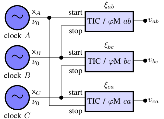
Fig. 1. Measurement principle. TIC stands for Time Interval Counter and φM for phasemeter.
