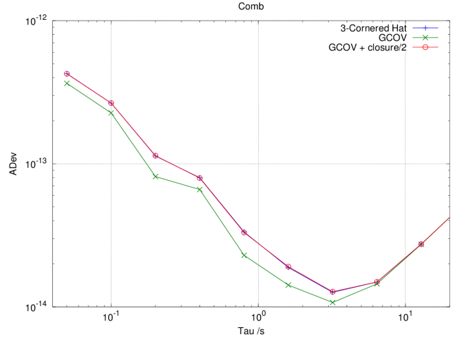
Fig. 4. Enlargement of the Allan deviation plot of the comb for the shortest time integrations obtained with the classical Three-Cornered Hat (blue) and with the Grosblambert Covariances (green). The difference between the estimates of the Allan variance of the comb obtained by these two methods is the Allan variance of the closure divided by 2.
